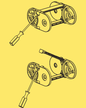
How to open the cover.
