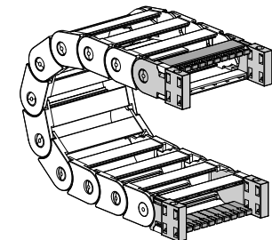
Fig. A Chain fixed outside/inside the radius. (Fig A)
