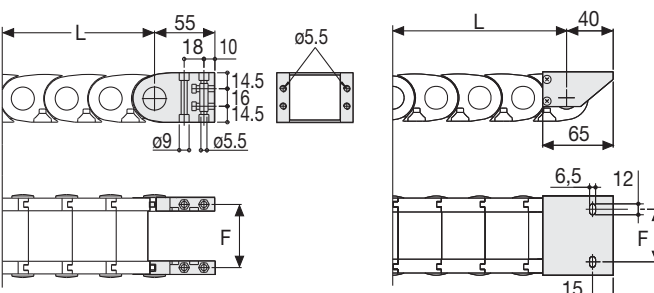
Fig. A The chain can be fixed frontally, inner or outer radius. (Fig A) Fig. B Chain fixed outside the radius. (Fig B) See end brackets mounting variations page 31.
