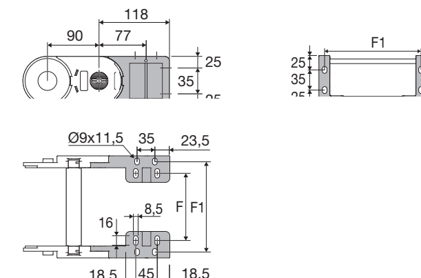
Fig. A The chain can be fixed frontally, inner or outer radius. (Fig A)
