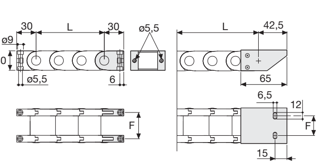
Fig. B Chain fixed outside the radius. (Fig B) See end brackets mounting variations page 31.
