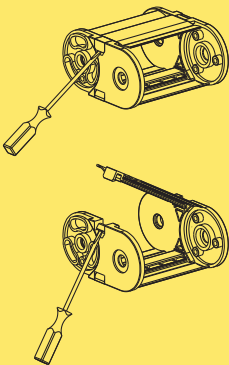
How to open the cover.
